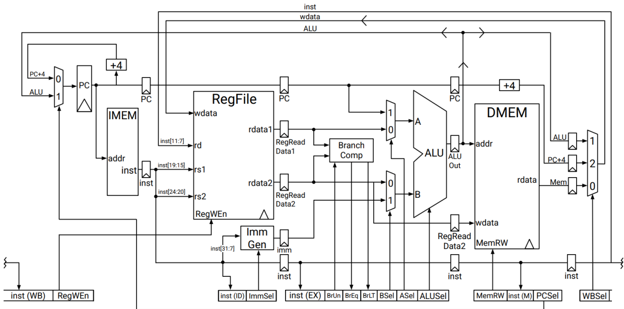
5-Stage Datapath Diagram
